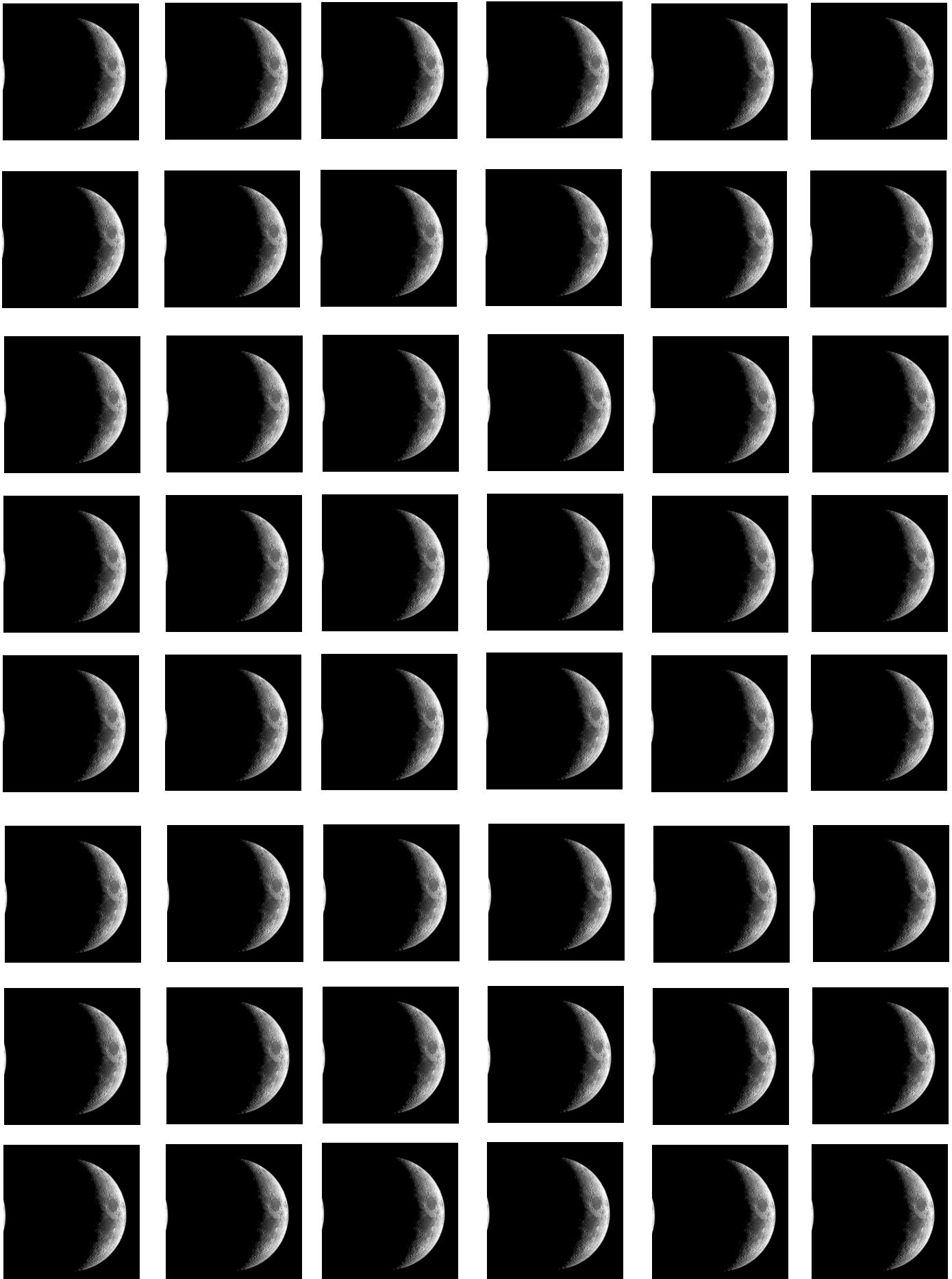
Waxing Crescent
