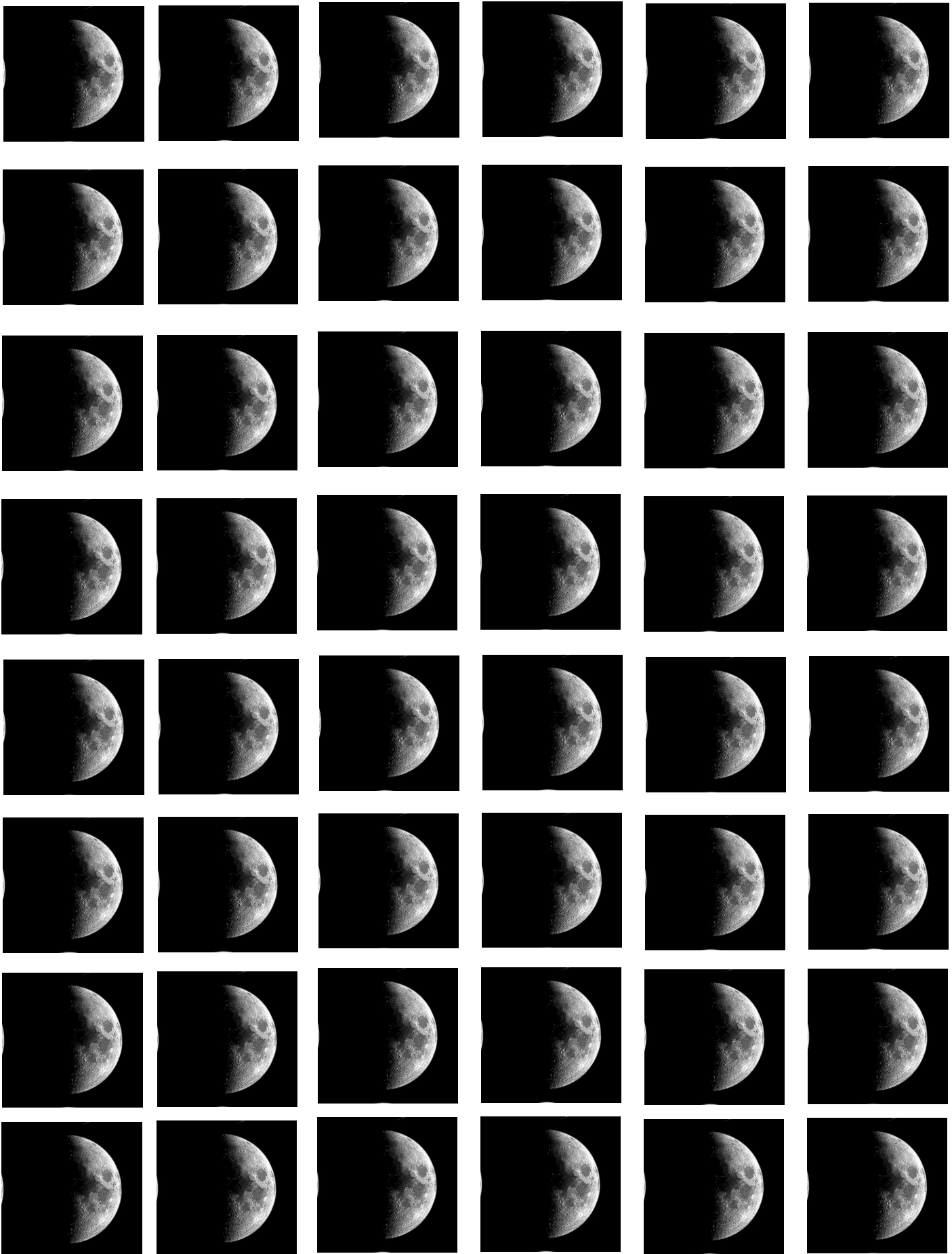
First Quarter
