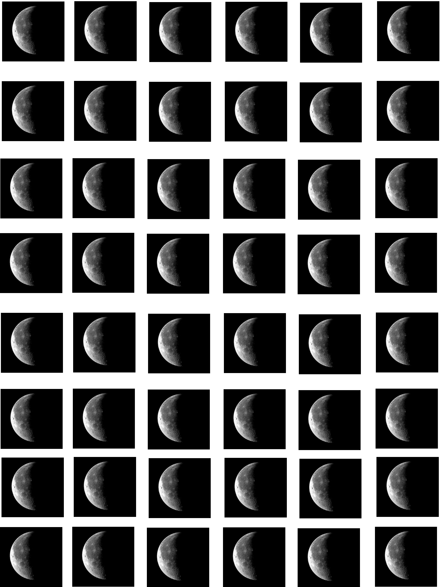
Waning Crescent
