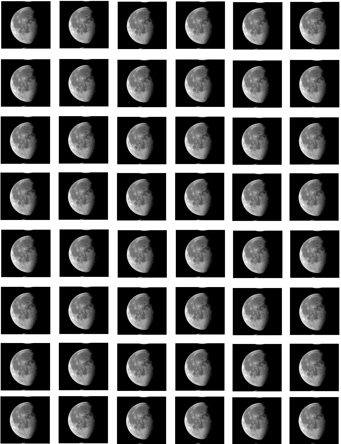
Last Quarter
