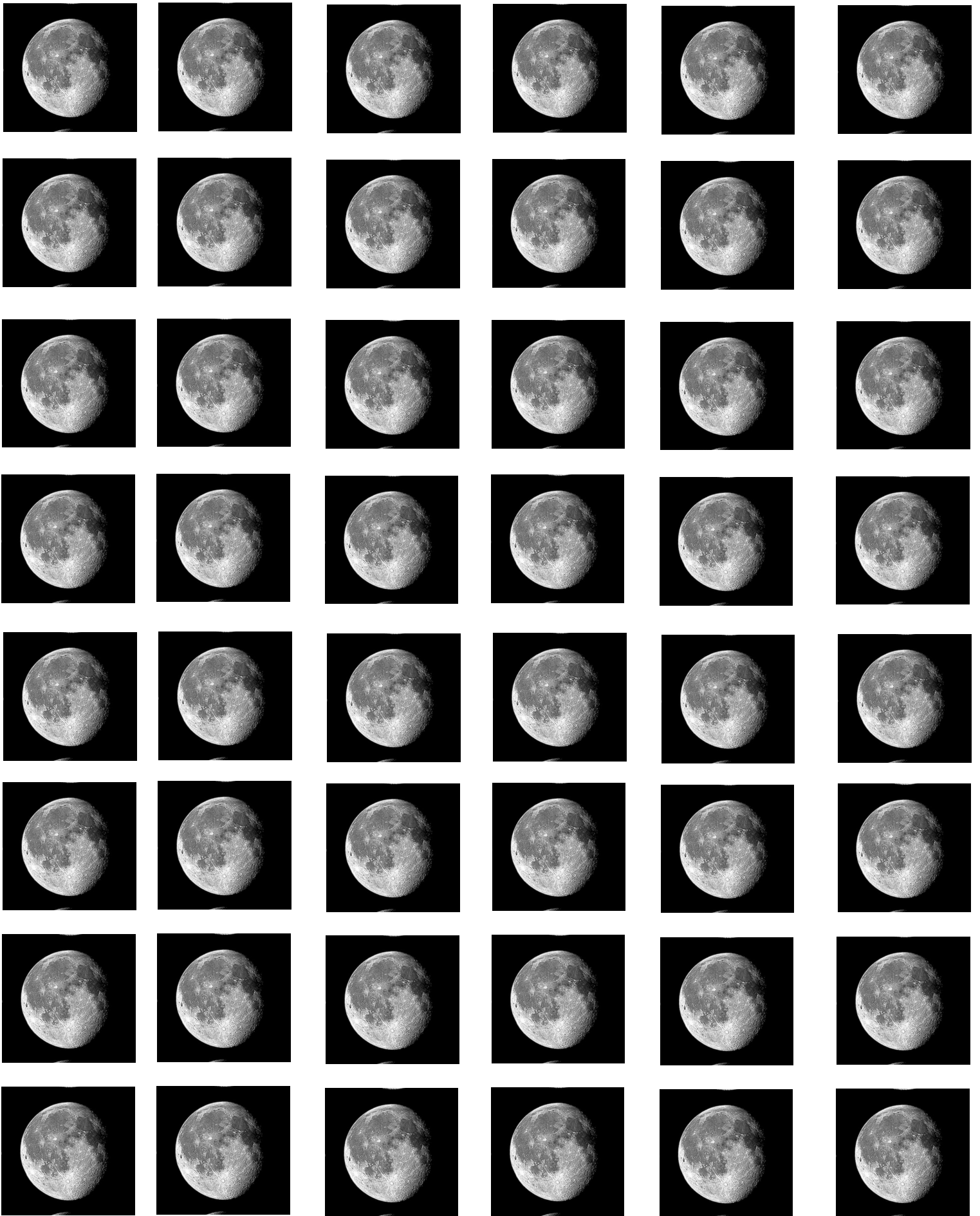
Waning Gibbous
